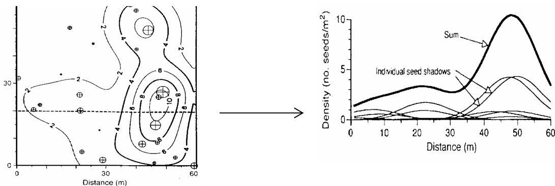
Figure: Example of source & seed distributions from a Temperate deciduous forest
